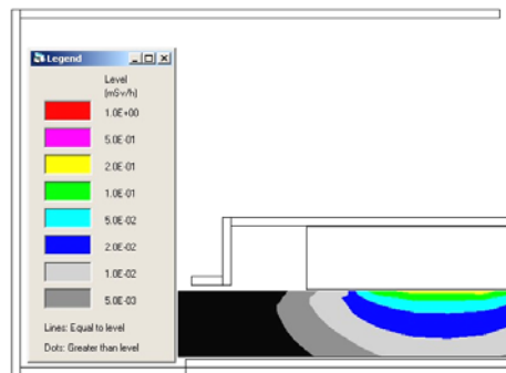
Fig. 4 : Estimation of dose rates inside the cell, via a grid, at the working place
