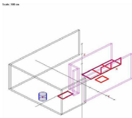
Fig. 3 : VISIPLAN Modelization cell 41
